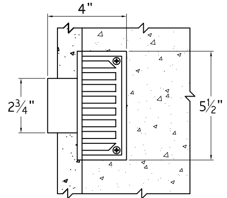
DRAIN DETAIL
