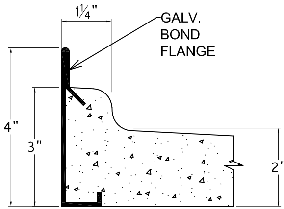
SECTION THRU SIDE SECTION 1
