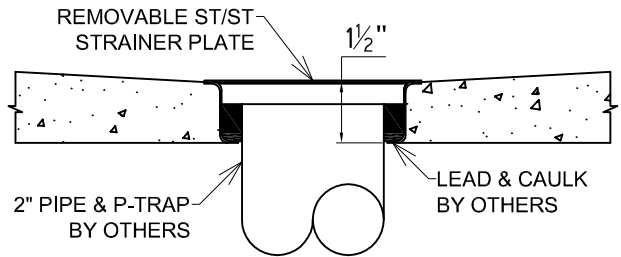
SECTION THRU DRAIN
